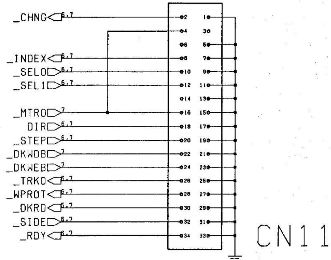
INTERNAL FLOPPY
