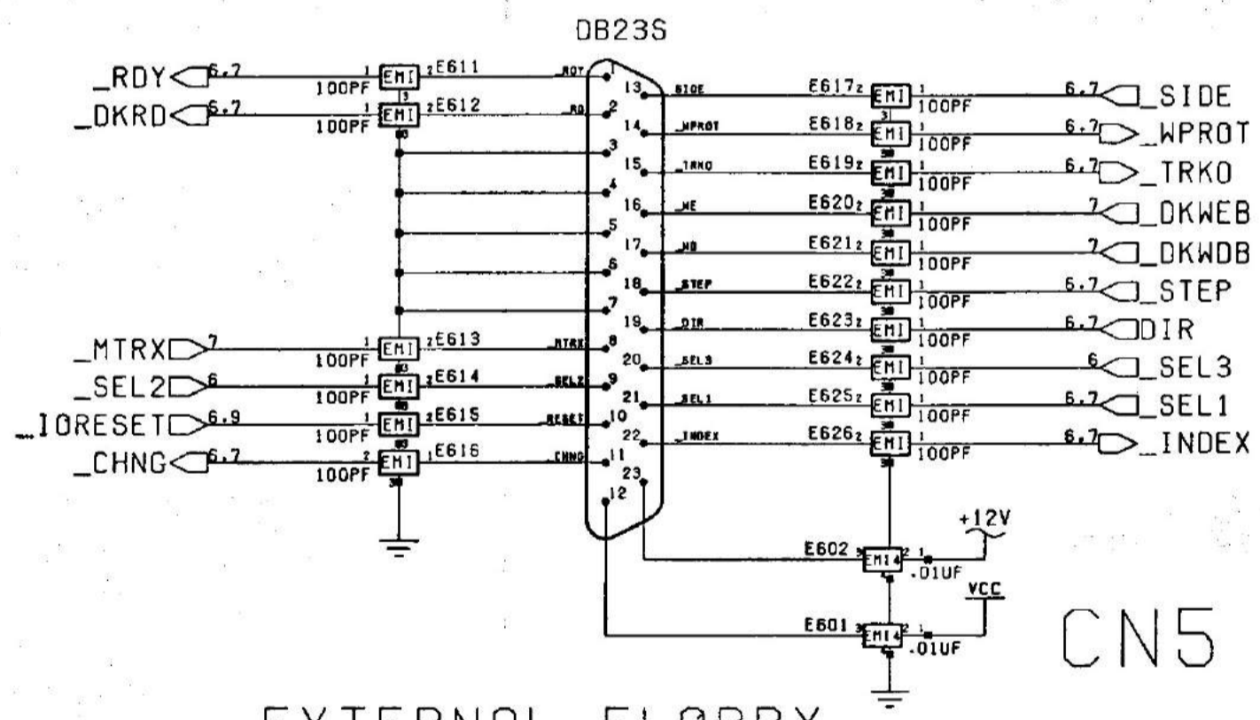
EXTERNAL FLOPPY
